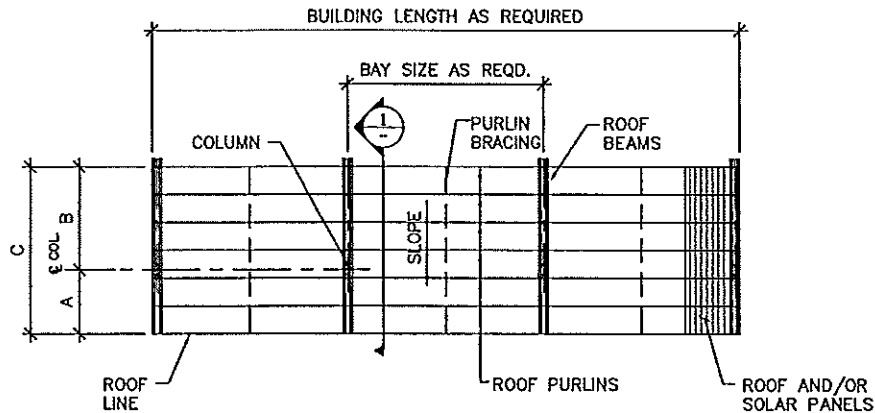
FRAMING PLAN
