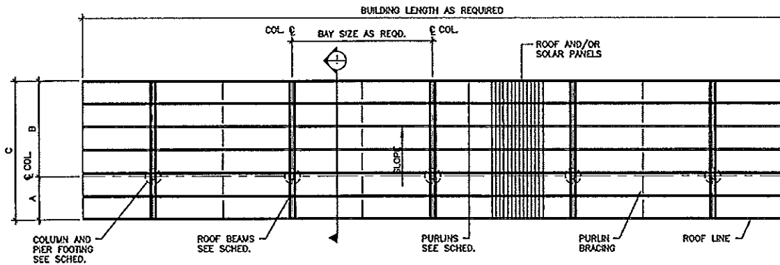
ROOF FRAMING PLAN
