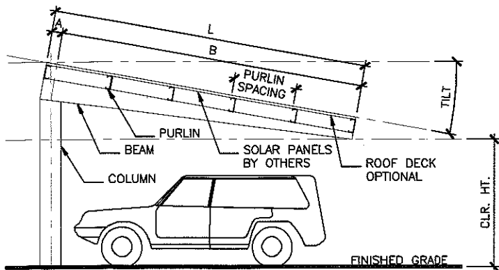
3 CROSS SECTION FC DOWN SLOPE N.T.S.
