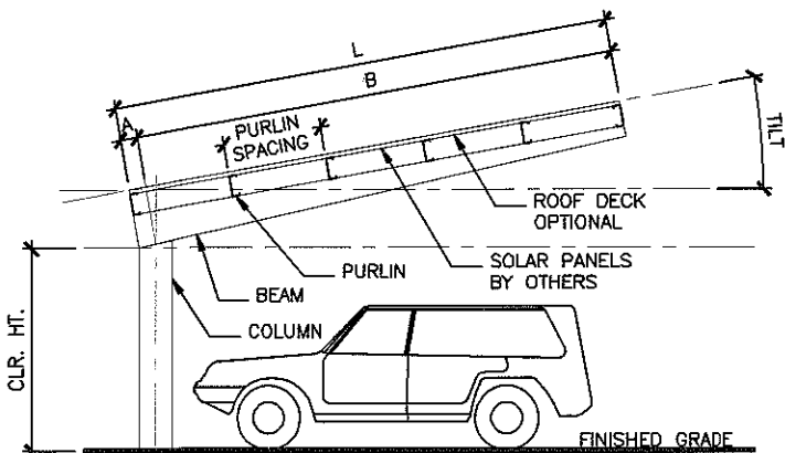
2 CROSS SECTION FC UP SLOPE N.T.S.
